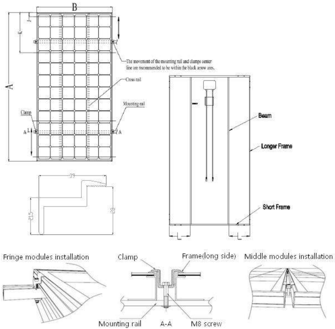
Figure 4: Light PV module installed at long side with Clamp fitting method
