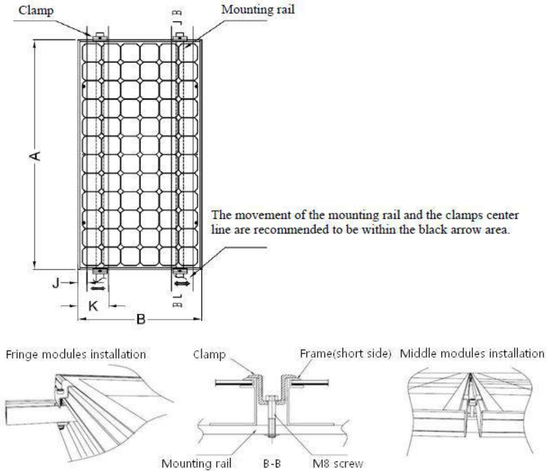
Figure 5: PV module installed at short side with Clamp fitting method
