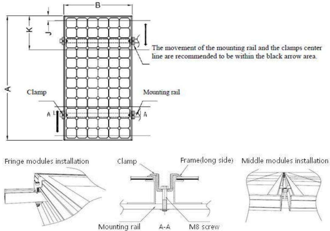
Figure 3: PV module installed at long side with Clamp fitting method
