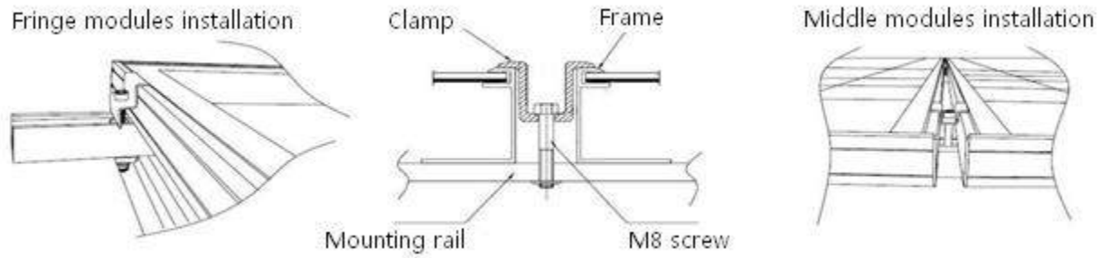
Figure 6: PV module installed at long and short side with Clamp fitting method
