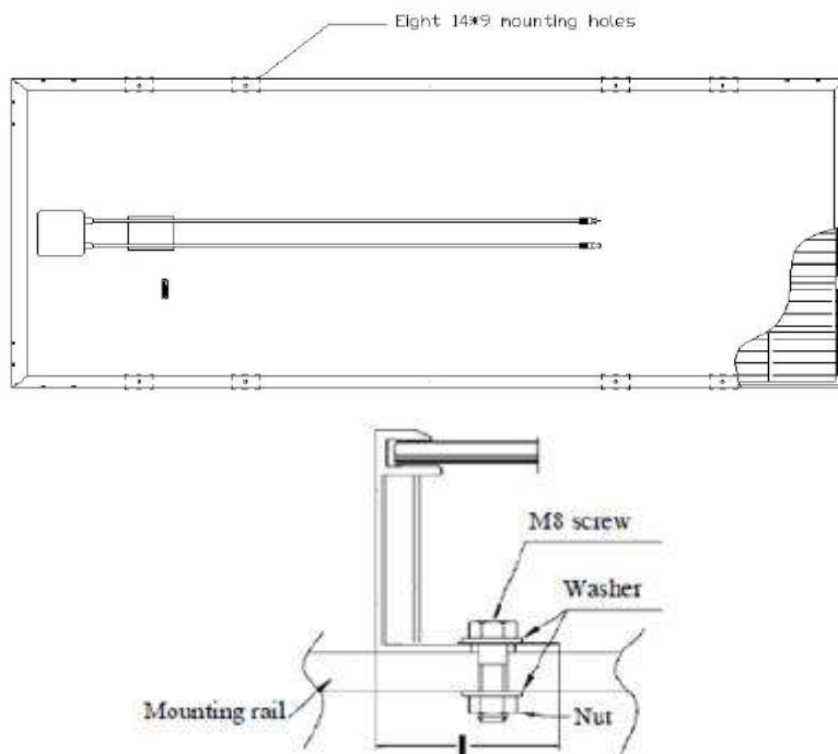
Figure 2: PV module installed with Screw fitting method
